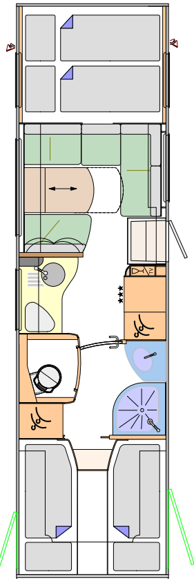
CRUISER IVECO 894 L EURO CARGO
